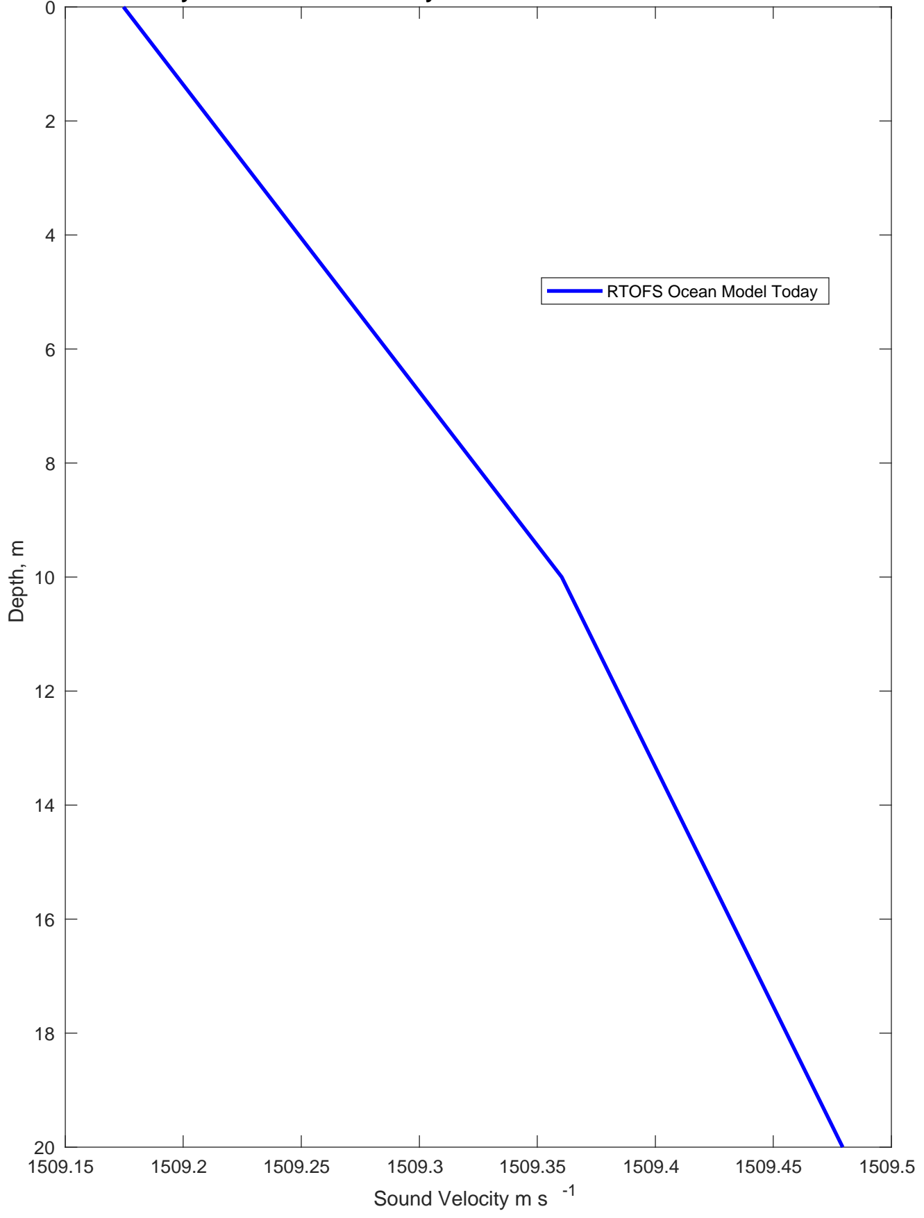
Sound Velocity Profile for US Wind Maryland Wind Farm on 08-Nov-2021 00:00:00
